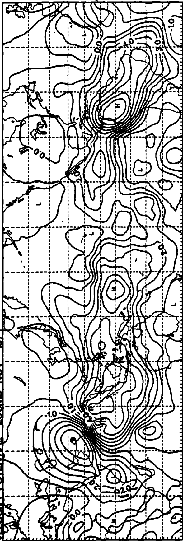
VELOCITY POTENTIAL 200MB NOV 1974
